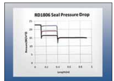
Finite Element Analysis to simulate the pressure drop across the three Wiper Seal Blades. This analysis helps in designing the geometry of each wiper seal.
